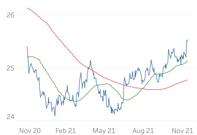
Currencies (UUP)
